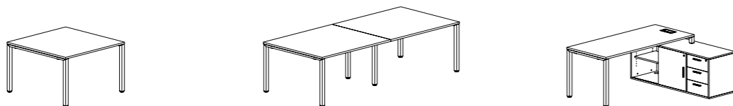
MEETING TABLE MESA REUNIÃO MESA REUNIÓN TABLE DE RÉUNION 1200/2000/2300 x 1200 x 740 MEETING TABLE MESA REUNIÃO MESA REUNIÓN TABLE DE RÉUNION 2800 x 1200 x 740 EXECUTIVE DESK POSTO DIREÇÃO PUERTO DIRECCIÓN BUREAU DIRECTION 1600/1800/2000 x 1600 x 740 2G . L / R
