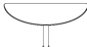
MEIA LUA P/ COMPACTOS 1200 X 600 X 740 | 1600 X 800 X 740 1236 X 618 X 740 | 1636 X 818 X 740
